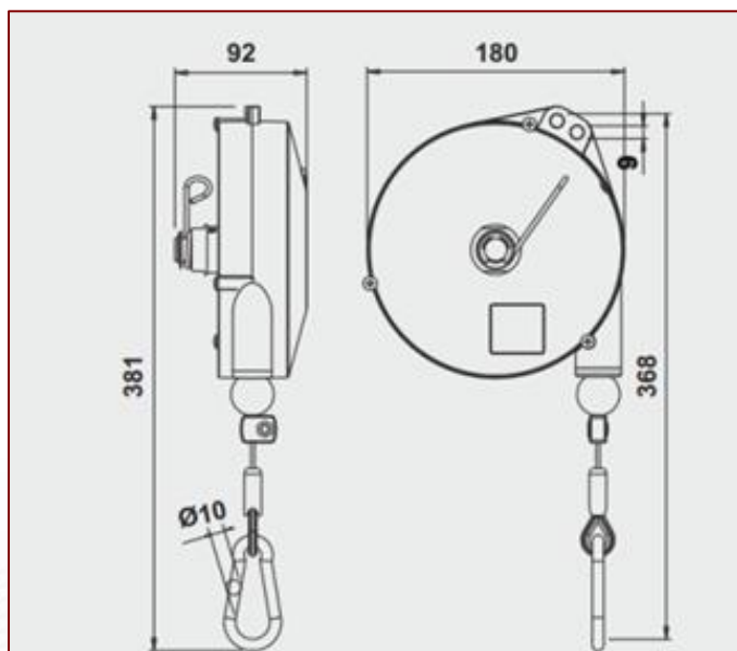
Plano dimensional Art. 9336-9340 / 9336NY-9340NY
