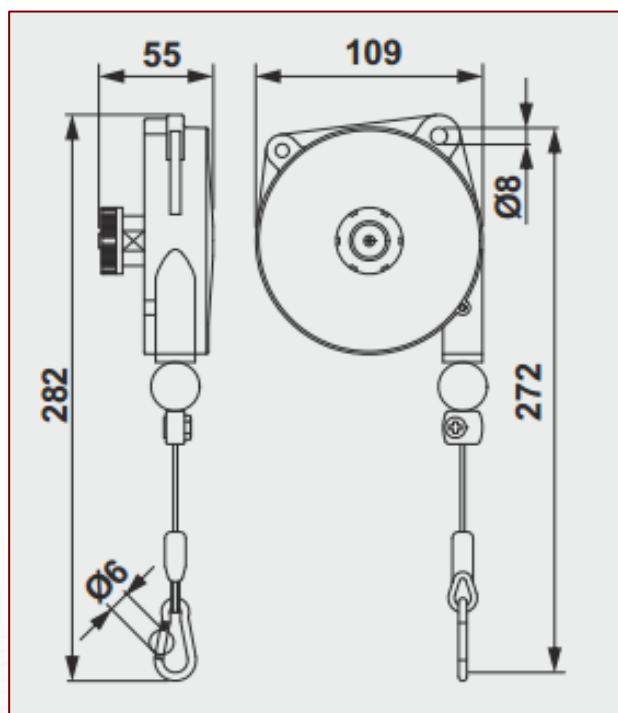
Plano dimensional 9311-9313 /9311NY-9313NY
