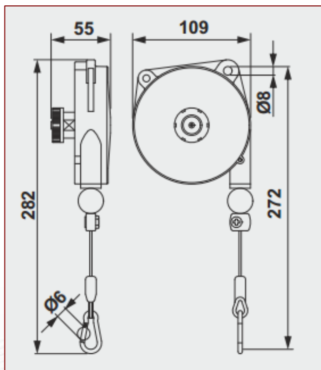
Plano dimensional 9300-9303 / 9300NY-9303NY
